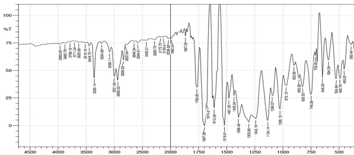
Fig 4: FTIR Spectrum of Apremilast
