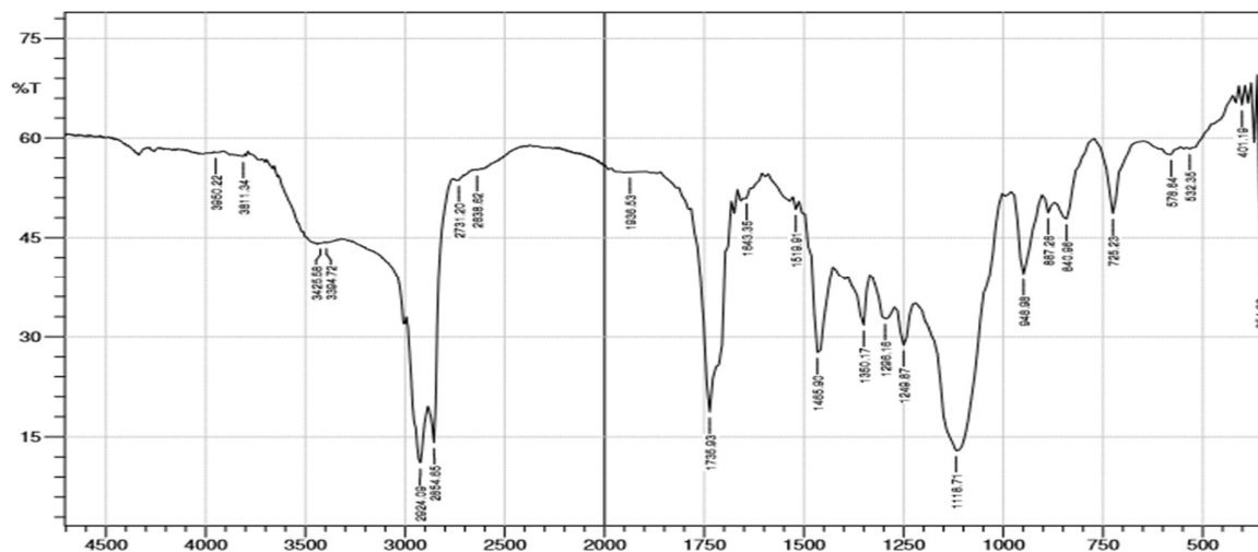
Fig 5: FTIR Spectrum of Apremilast with Physical Mixture
