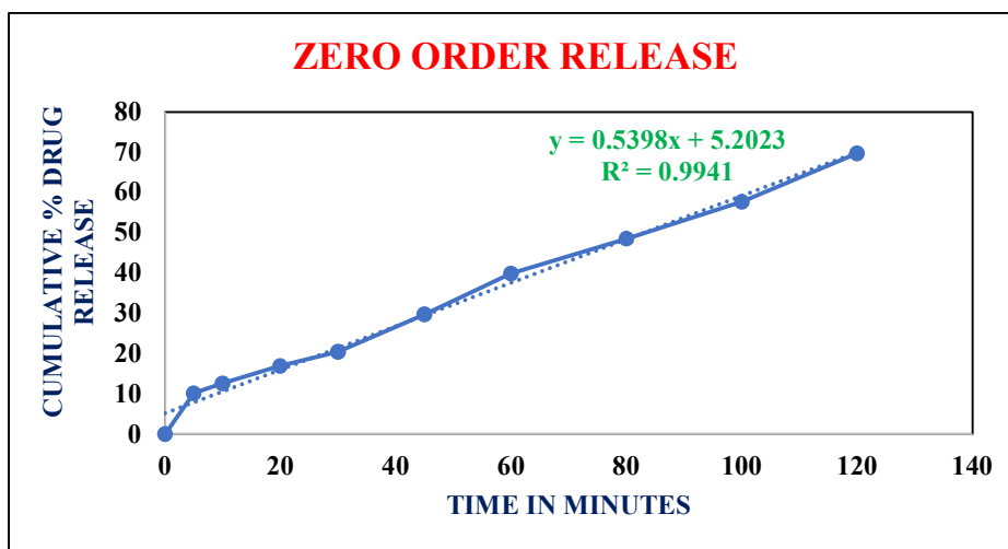
Fig 12: Zero Order Release Kinetics
