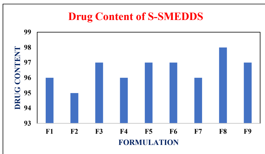
Fig 8: Graphical Representation of Drug Content of S-SMEDDS
