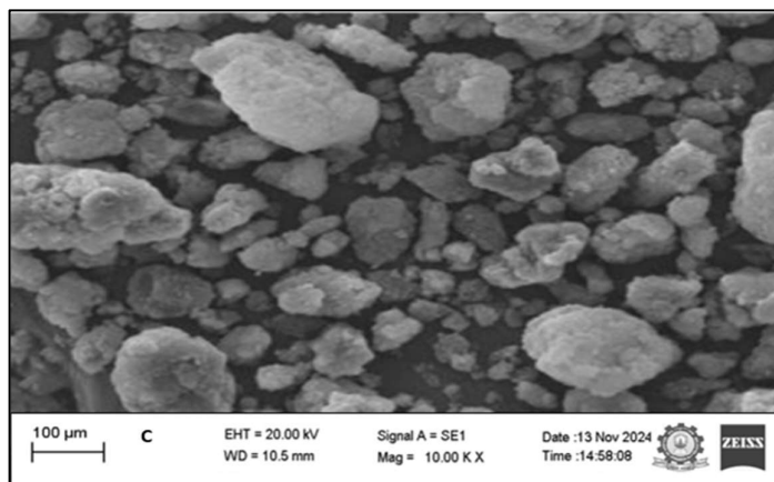
Fig 23: SEM image of Apremilast Loaded S-SMEDDS in Various Magnification
