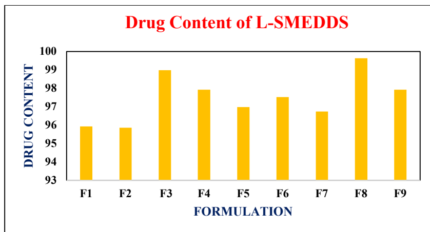
Fig 7: Graphical Representation of Drug Content of L-SMEDDS
