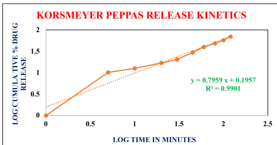
Fig 15: Korsmeyer Peppas Release Kinetics
