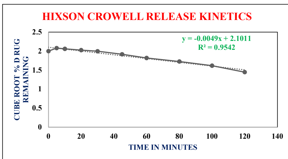
Fig 16: Hixson Crowell Release Kinetics
