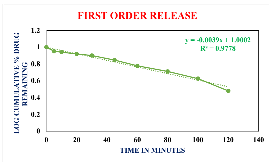
Fig 13: First Order Release Kinetics
