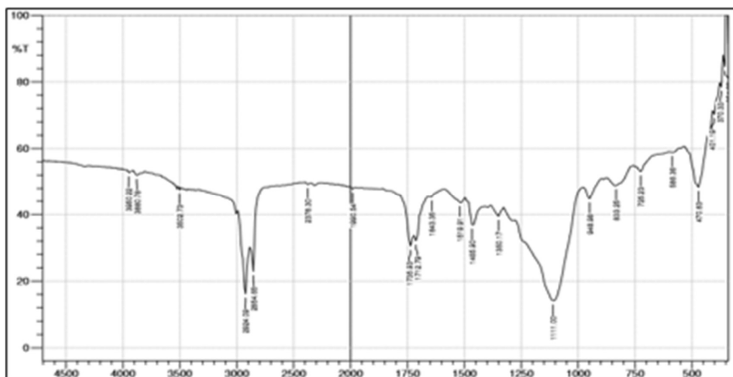
Fig 17: FT-IR Spectrum of Best Formulation
