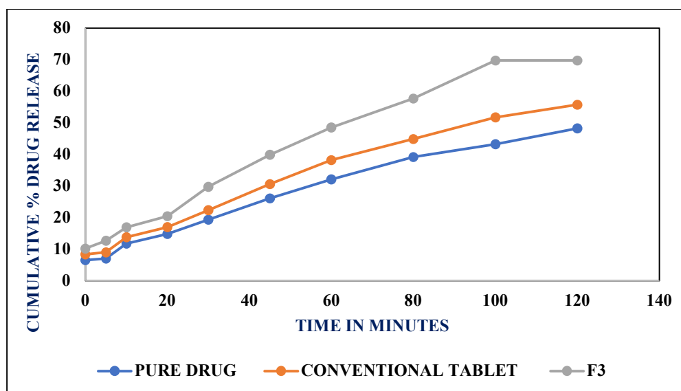
Fig 11: Comparison of In Vitro Drug Release of Pure Drug, Conventional Tablet and Best SMEDDS Formulation (F3)
