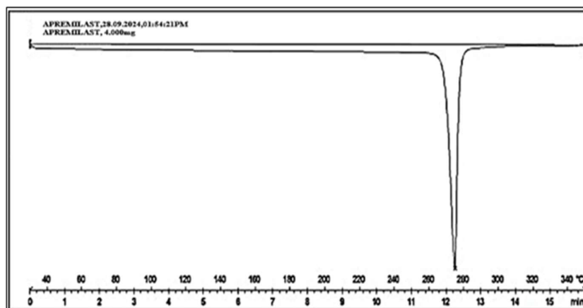
Fig 20: DSC Thermogram of Pure Apremilast
