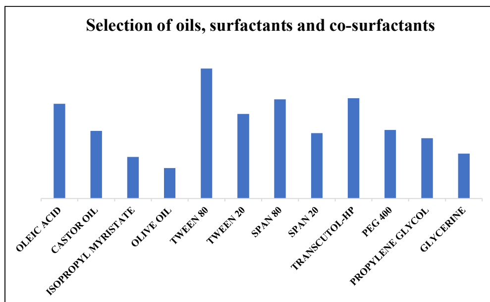
Fig 3: Solubility of Apremilast in various oils, surfactants, and cosurfactants
