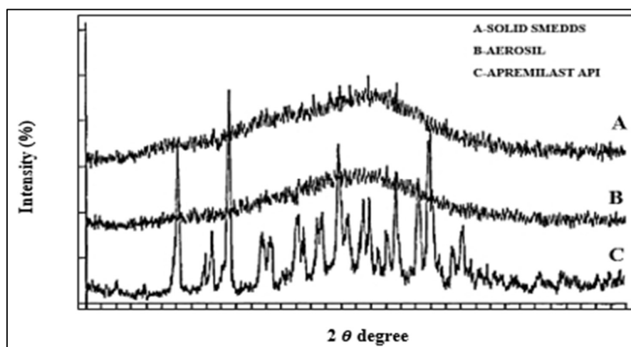
Fig 22: XRPD Pattern of Pure Drug, Aerosil & S-SMEDDS
