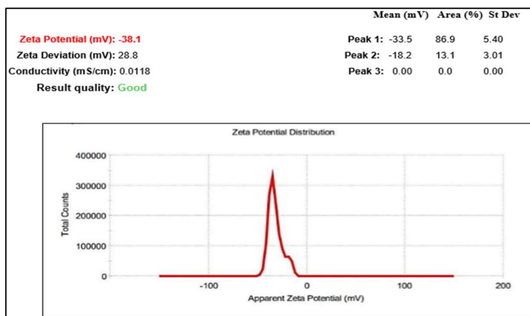
Fig 19: Zeta potential determination of best formulation F3
