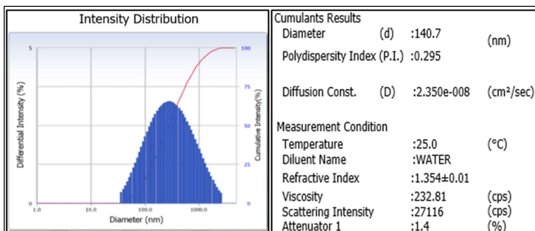
Fig 18: Mean globule size and size intensity distribution graph of best formulation F3
