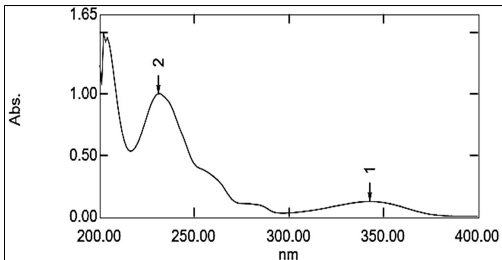
Fig 1: Determination of \lambda_{\text{max}} of Apremilast
