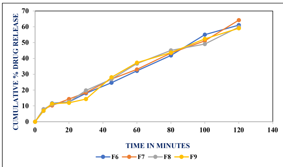
Fig 10: In-Vitro Drug Release studies of Formulations F6, F7, F8 and F9
