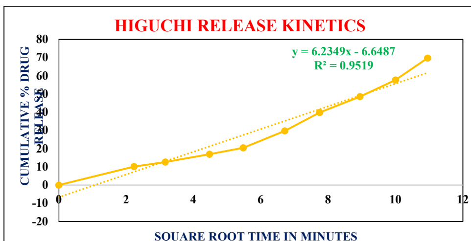
Fig 14: Higuchi Release Kinetics
