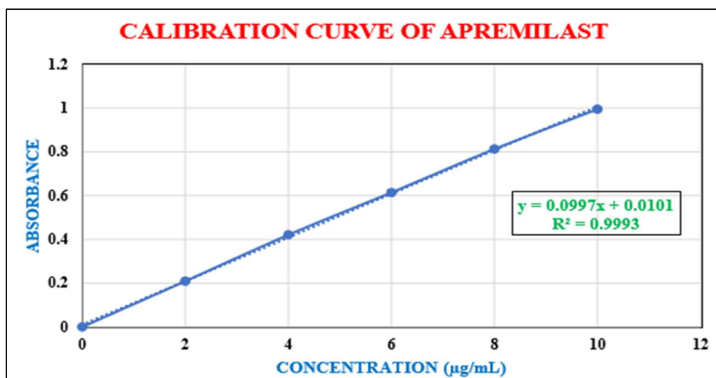
Fig. 2: Calibration curve of Apremilast
