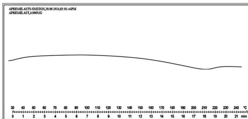
Fig 21: DSC Thermogram of Apremilast S-SMEDDS
