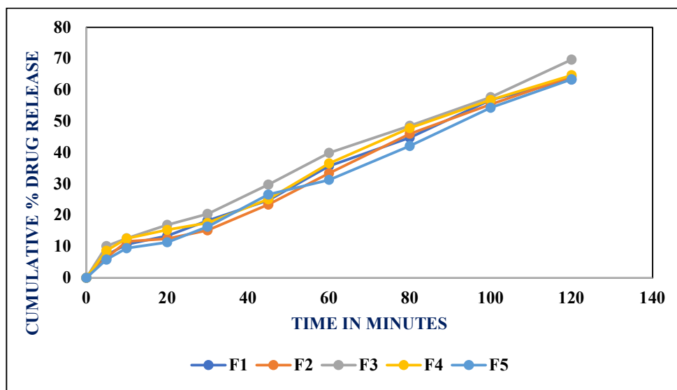
Fig 9: In-Vitro Drug Release studies of Formulations F1, F2, F3, F4 and F5
