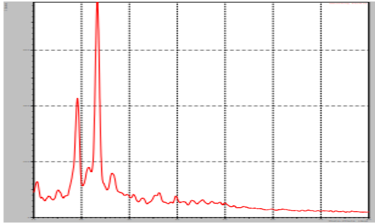
Fig5: XRDRosuvastatinR6nanoparticles
